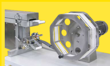
yarn tension control (compensator arm) and reel for up to 4 yarns
